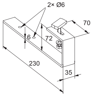
c) Stainless steel roof anchor for metal or slate roofing steel for pantiles
