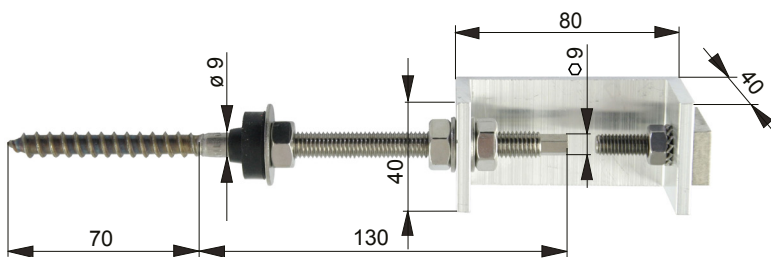
d) Roofing bolt for rail fixing
