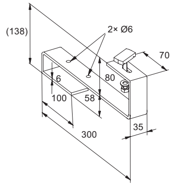
b) Roof anchor of stainless steel or zinc-plated steel for pantiles
