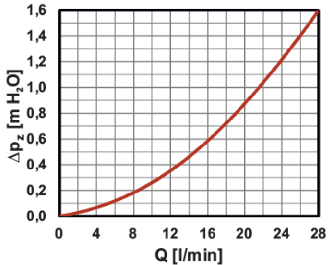
Flowmeter · 8-28 l/min
