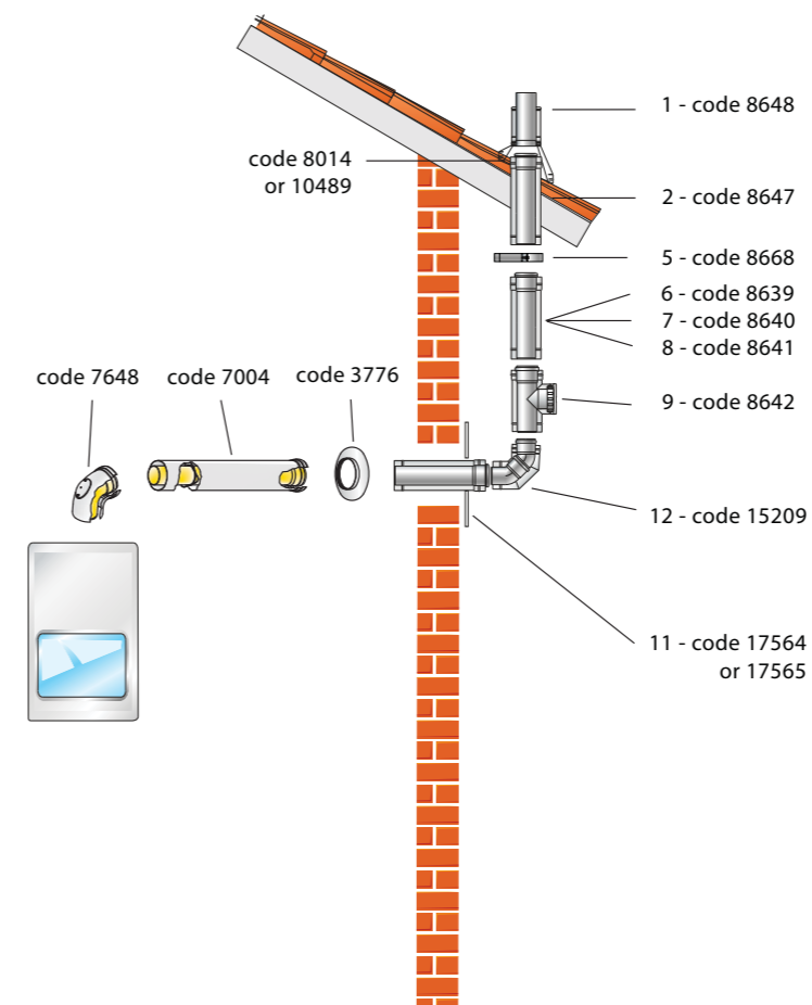
External flue gas discharge using concentric elbow and combustion air intake through vertical terminal
