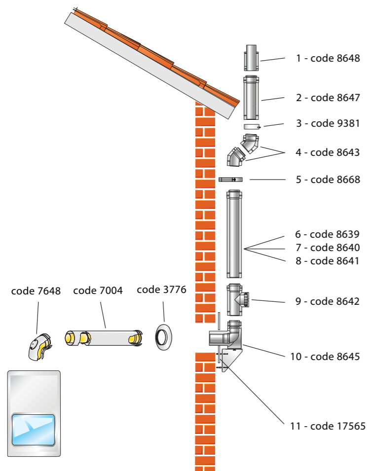
External flue gas discharge using elbow w. support and combustion air intake
